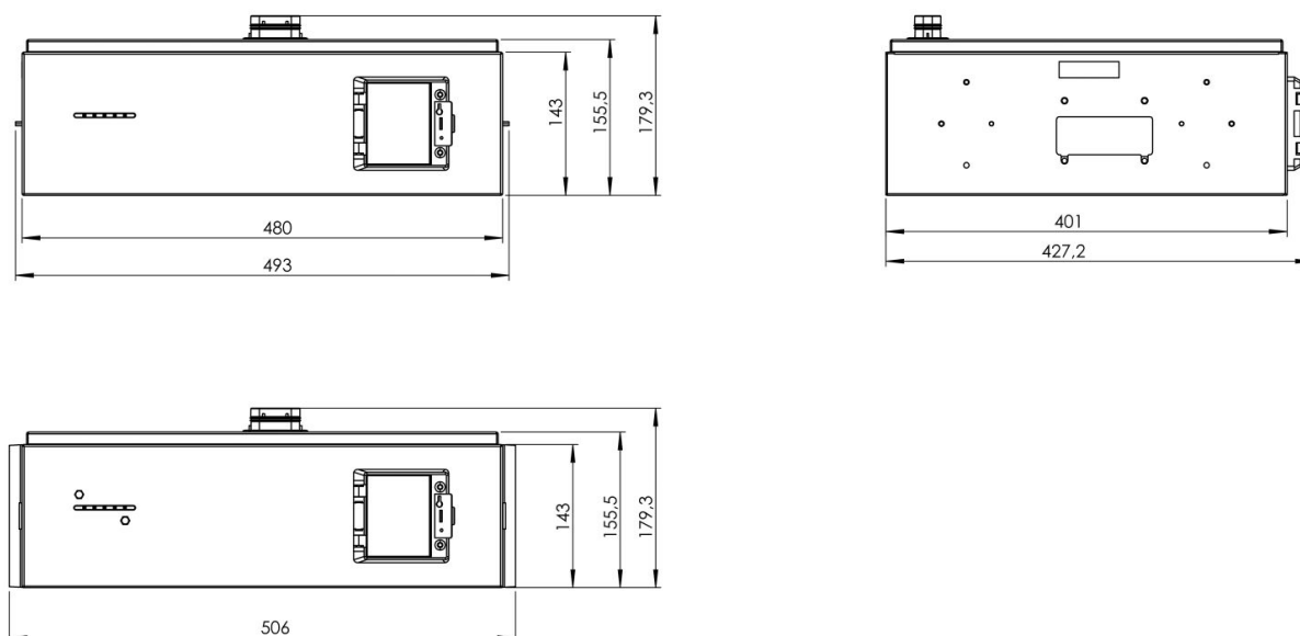
Image 8. Dimensions — BMS box
