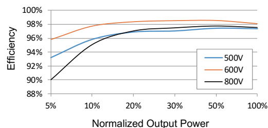
EFFICIENCY CURVE (SG33CX-P2)
