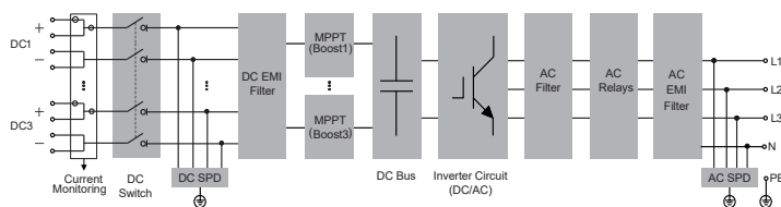
CIRCUIT DIAGRAM (SG33CX-P2)
